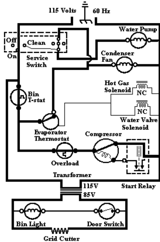
ICE MAKING CYCLE
