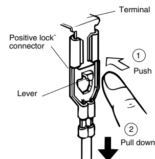
Positive lock® connector
