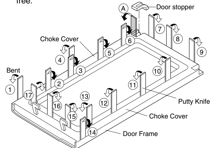
Figure C-3. Door Disassembly
