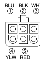
6-PIN CONNECTOR OF HOOD FAN MOTOR
