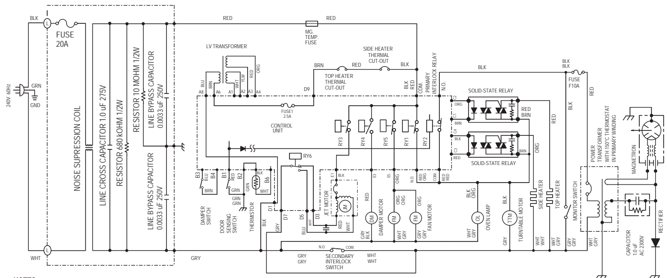
Figure O-5. Oven Schematic-Speed Roast Cooking Condition
