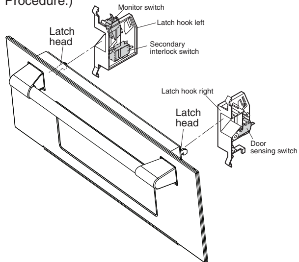
Figure C-3. Latch Switch Adjustment
