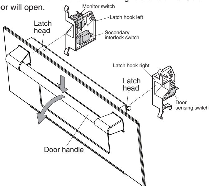
Figure D-1. Door Open Mechanism
