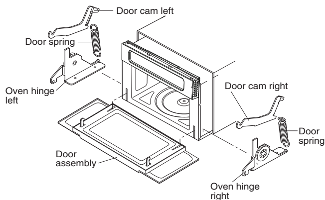
Figure C-4(a). Door Replacement
