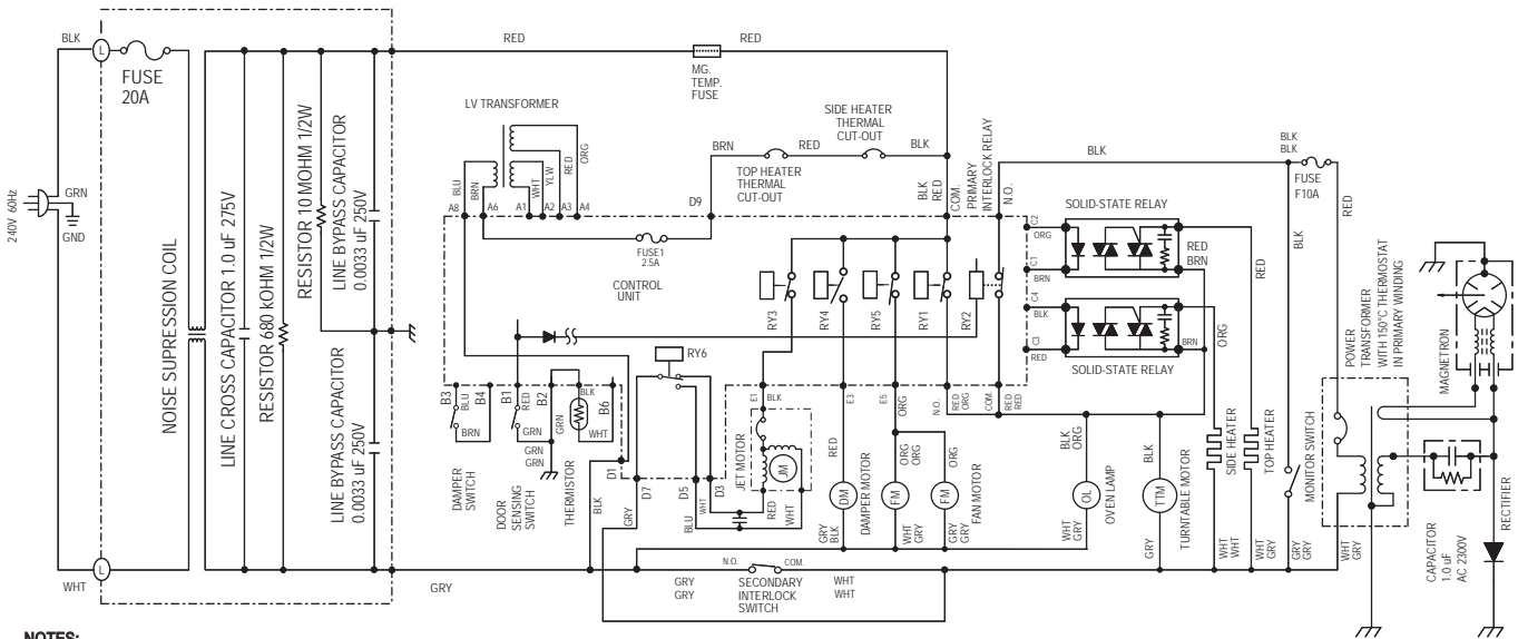
Figure O-4. Oven Schematic-Speed Grill Cooking Condition
