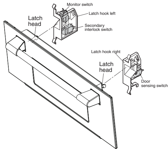
Figure C-2. Switches
