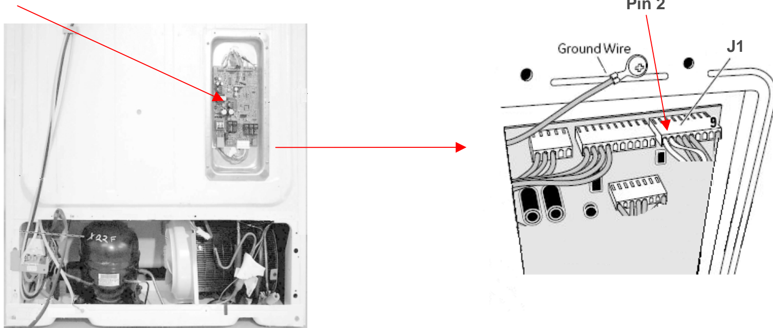
Vertically Mounted Control Board
