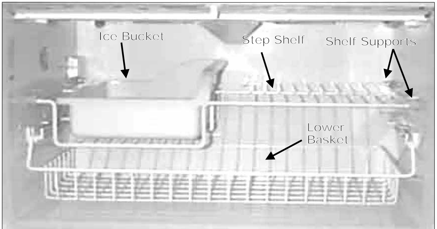
FINAL ASSEMBLY OF STEP SHELF KIT (Icemaker not installed in picture)
