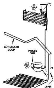
SEALED SYSTEM
