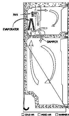
AIR FLOW
