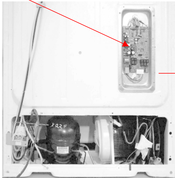
Vertically Mounted Control Board
