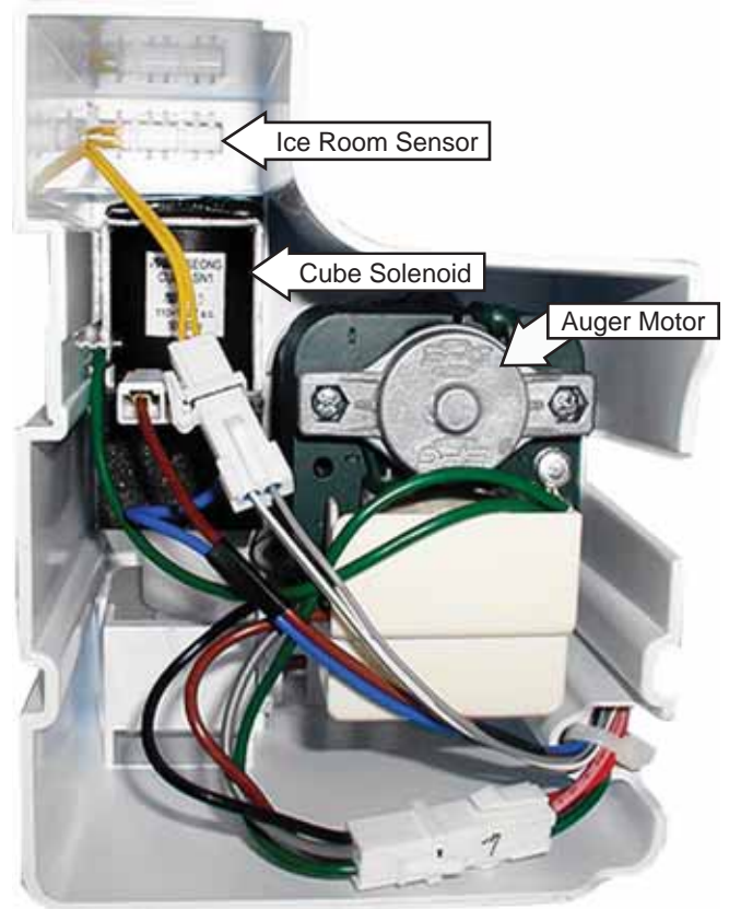
Auger Assembly Components
